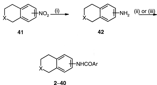
Scheme 1. Reagents and conditions: (i) 10% Pd/C, H 2 , ethanol, 4 h, > 90% yield; or SnCl 2 , EtOH, 3 h, 50 °C, 40–60% yield; (ii) ArCOCl, Et 3 N, CH 2 Cl 2 , 6 h, 25 °C, 45–85% yield; (iii) ArCO 2 H, 1-(3-Dimethylaminopropyl)-3-ethylcarbodiimide, HOBT, DMF, 18 h, 25 °C, 50–85% yield.
