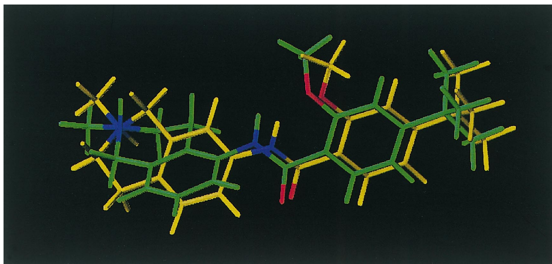
Figure 1. Overlapped energy minimised conformations of 6 (green) and 28 (yellow) generated using the SYBYL package (O = red, N = blue).
