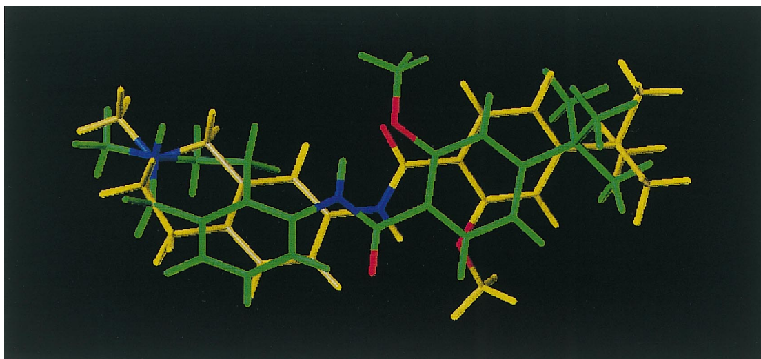
Figure 2. View of the alternative overlapped energy minimised 6 (green) and 28 (yellow) generated using the SYBYL package (O = red, N = blue).
